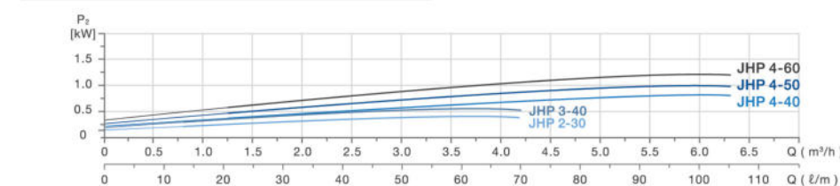
Power (P 2 ) Vs. Volume
