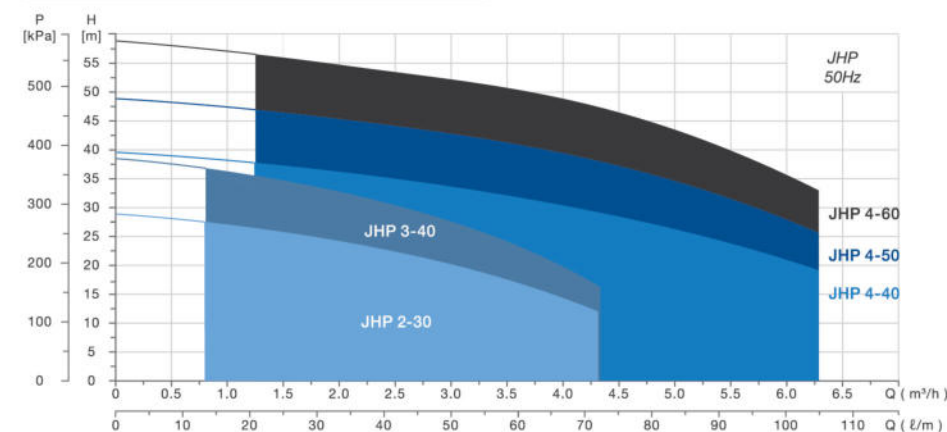
Pressure / Height Vs. Volume
